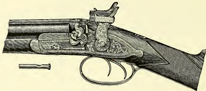
Joseph Manton's "Tube" Detonating Gun.
